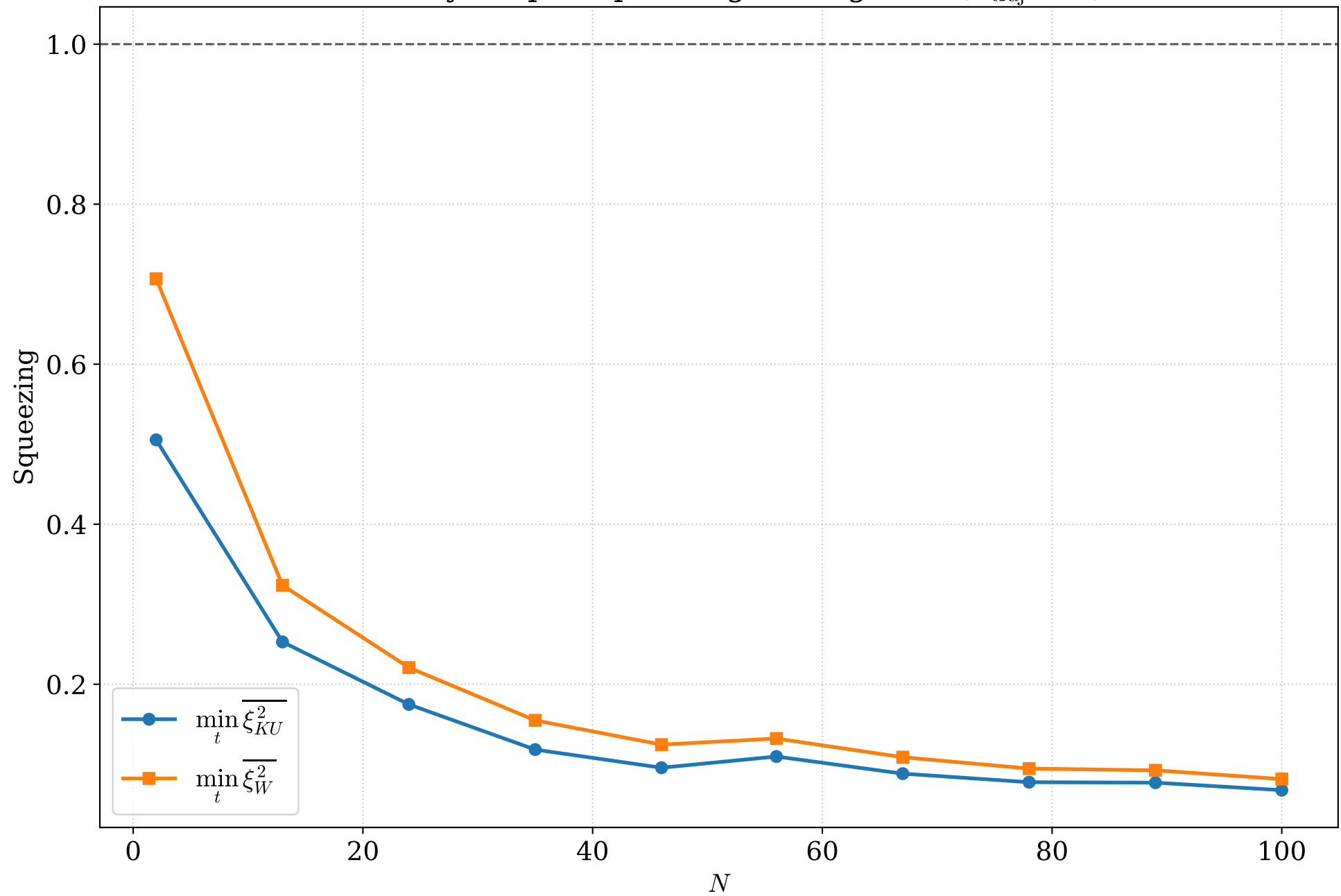
Homodyne spin-squeezing scaling vs N ( n_{\text{traj}}=50 )
